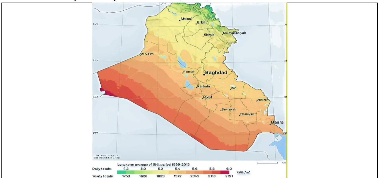
Fig. 2. Global horizontal irradiation (GHI) Solar radiation Iraq [29].
