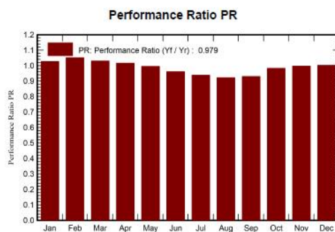
0.95 albedo
