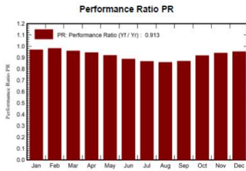
0.6 albedo
