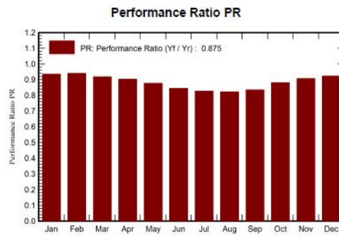
0.4 albedo
